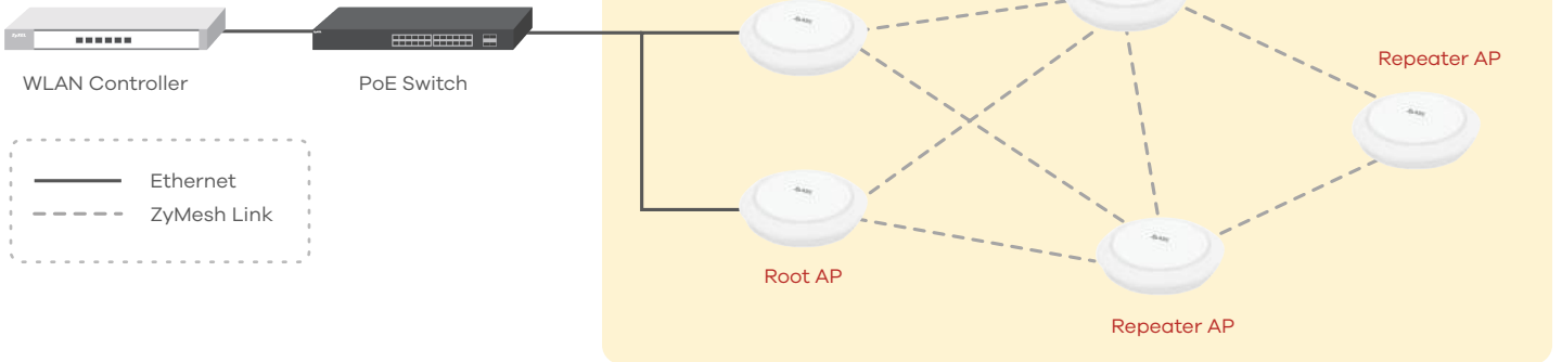
Application Diagram ZyMesh
